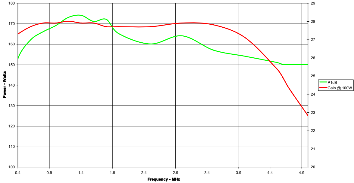
Gain and P1dB
